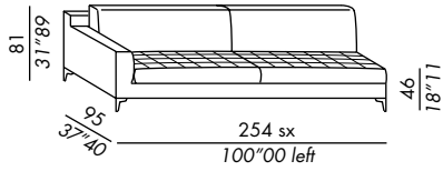
terminale / end unit QUILT 255
