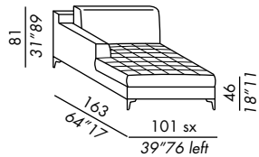
chaise longue QUILT
